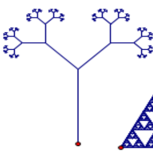
Binary Tree
