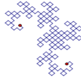
Dragon Fractal
