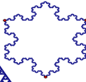
Koch Snowflake
